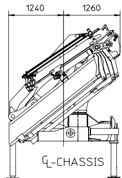
3450-K + fly-jib FJ900
