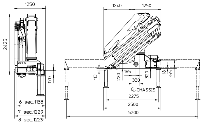
3450-K + fly-jib FJ900
